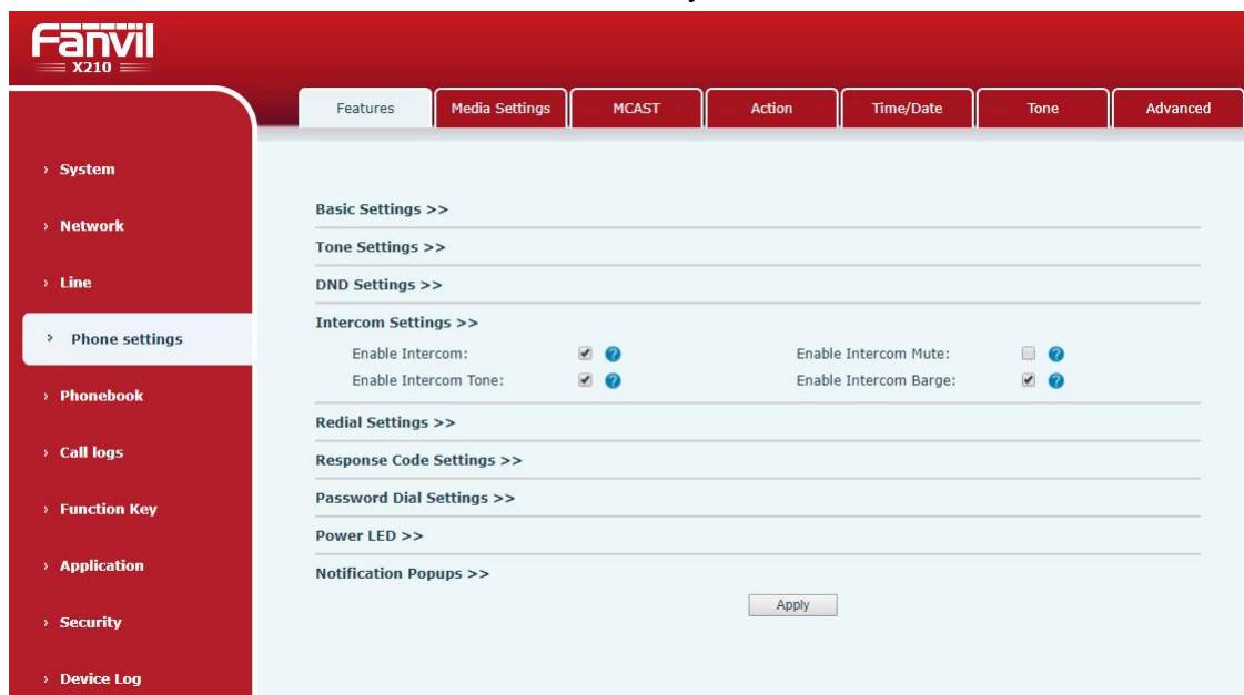
Picture 72 - Web Intercom configure
