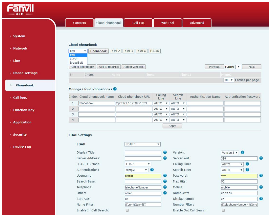
Picture 136 - Web cloud phone book Settings
